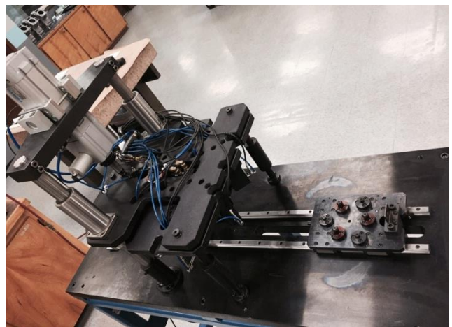
Automatic Gages
